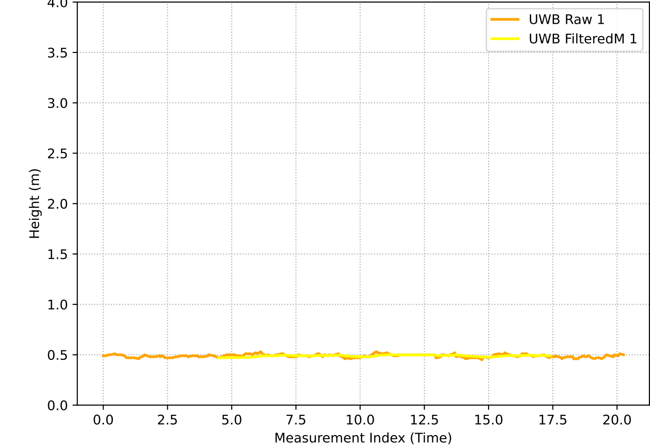
Z-Axis (Altitude) Stability Profile
